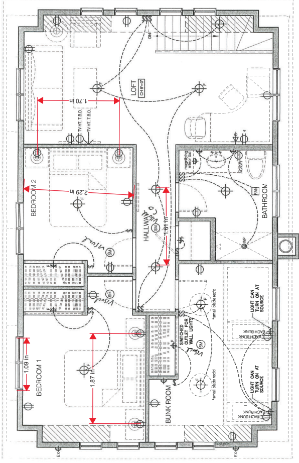
UPPER RCP AND ELECTRICAL PLAN
